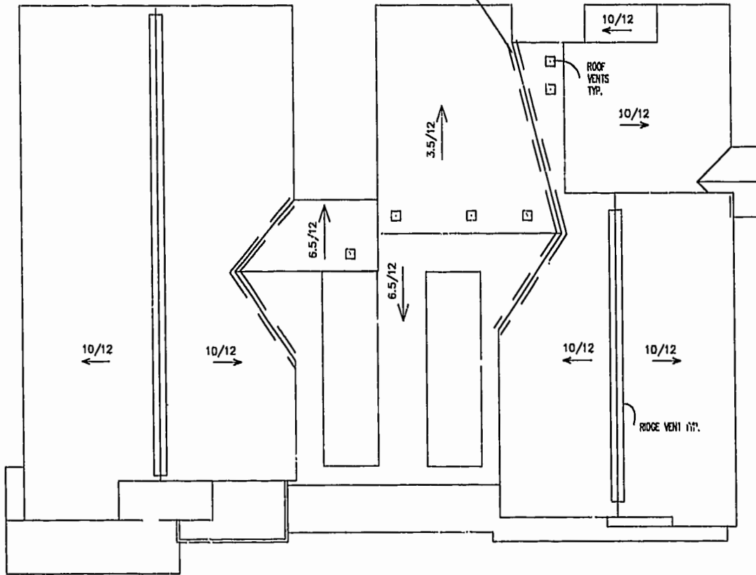
ROOF PLAN
