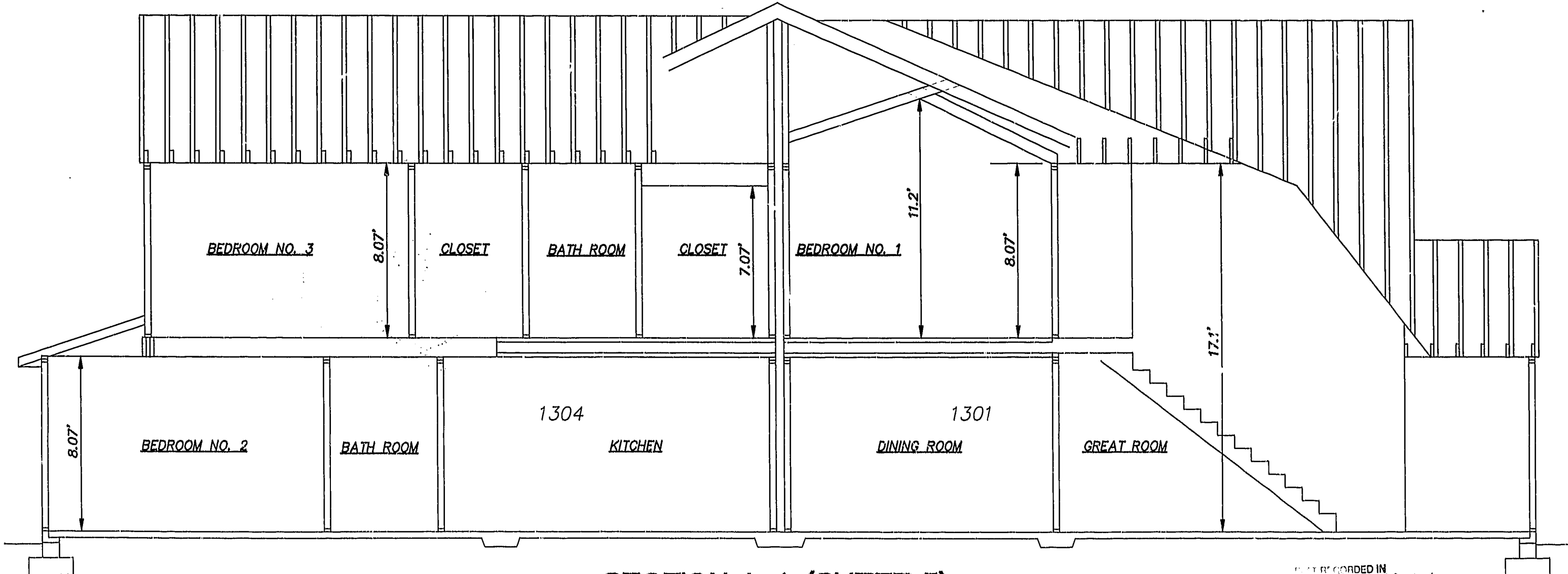
SECTION A-A (SHEET 5)
