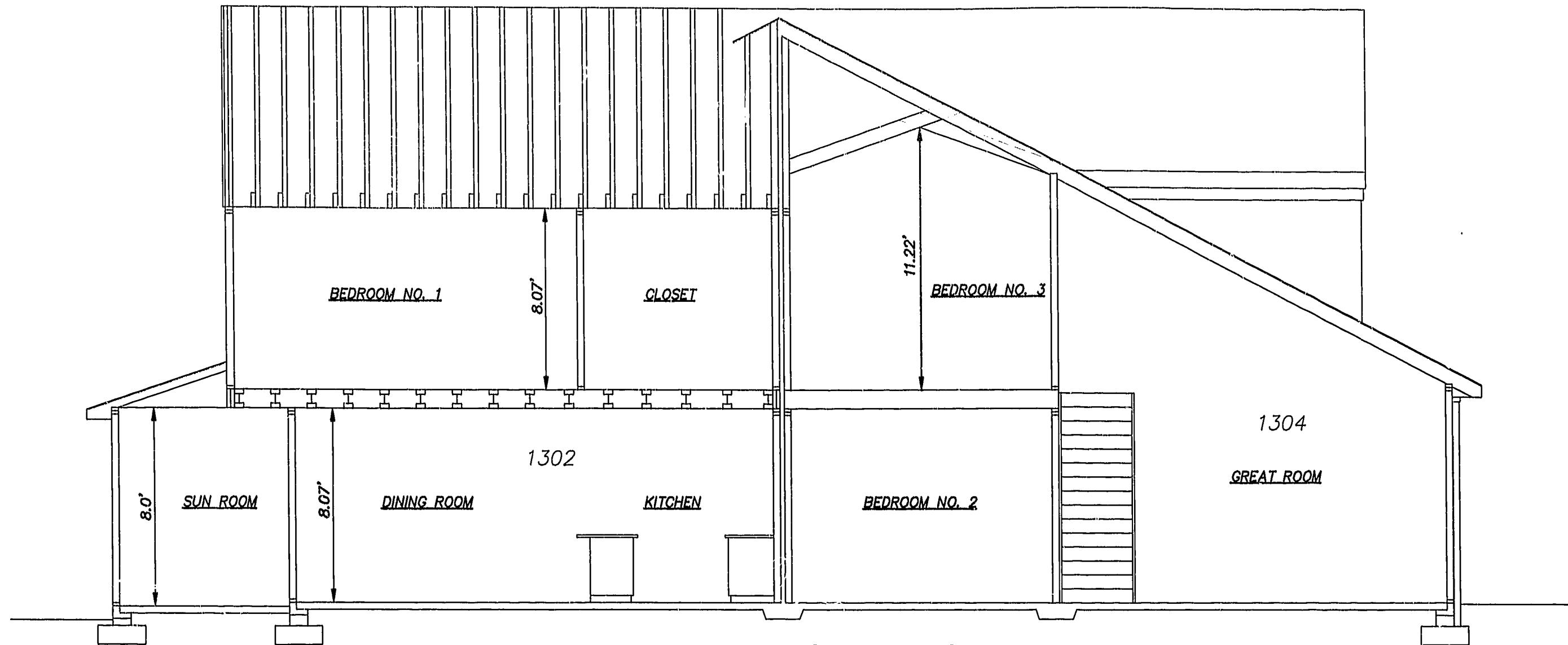
SECTION B-B (SHEET 5)
