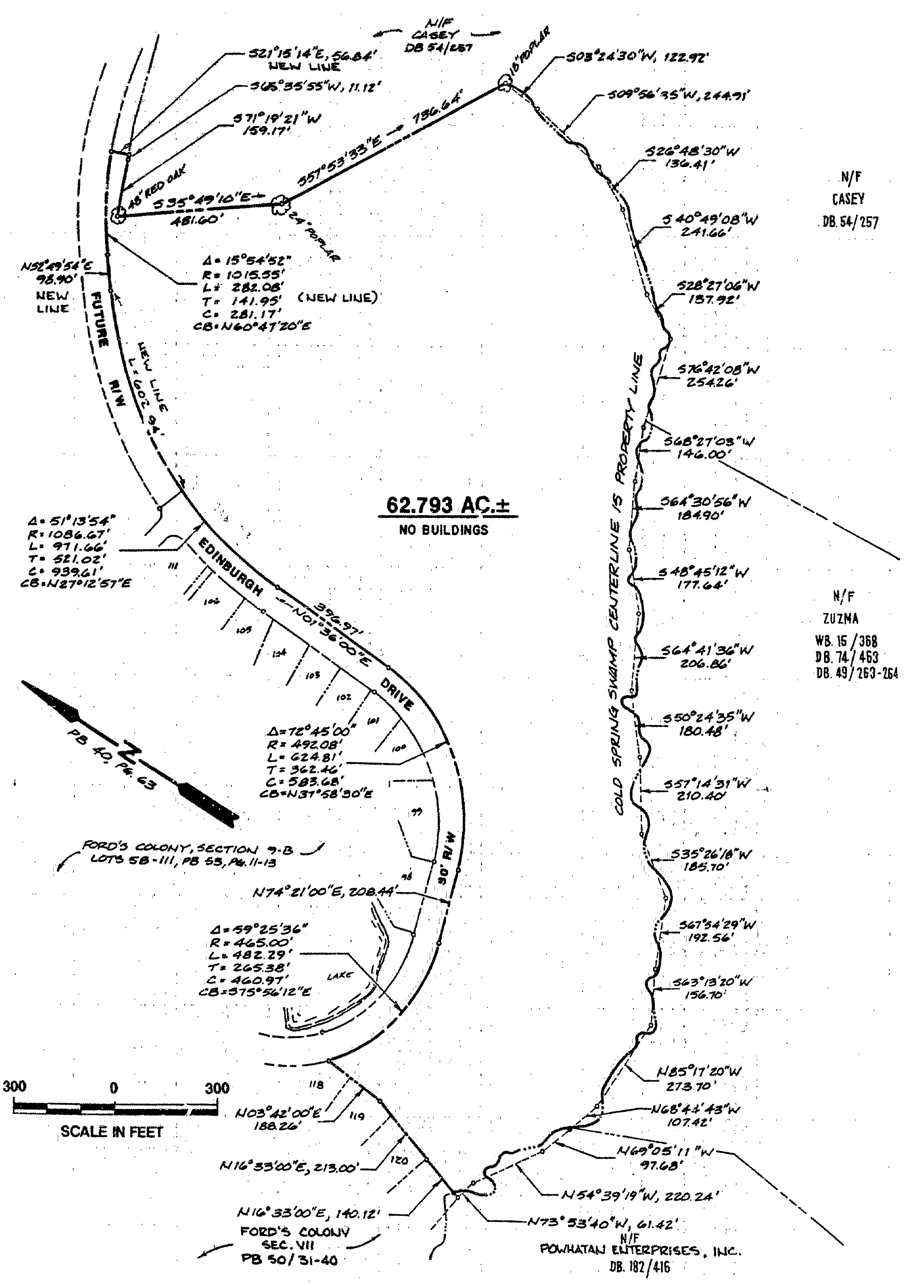
PERIMETER SURVEY OF FORD'S COLONY @ WILLIAMSBURG SECTION IX-A (A-9a)
