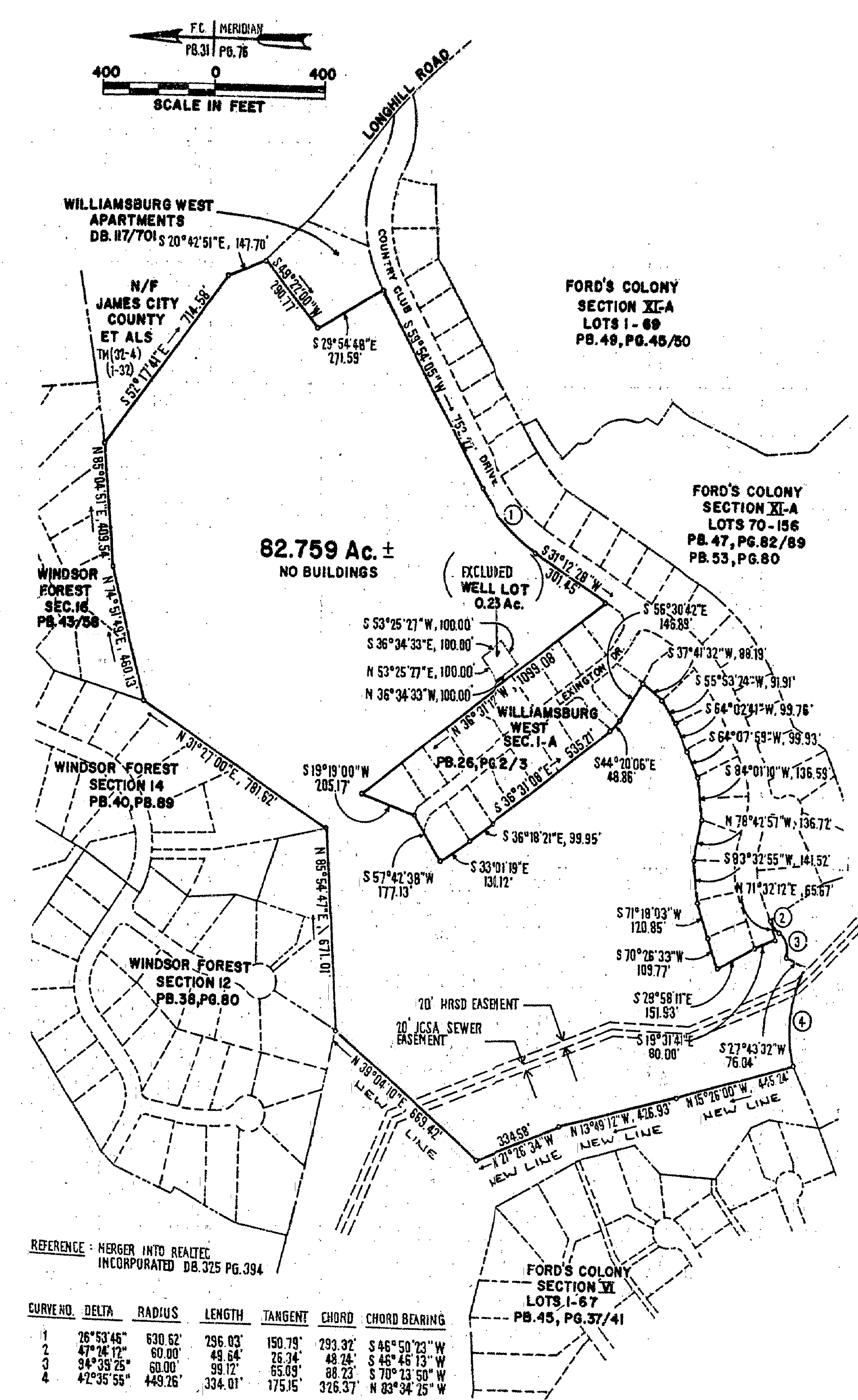
PERIMETER SURVEY OF FORD'S COLONY @ WILLIAMSBURG SECTIONS XII (A-12) & XV (A-15)
