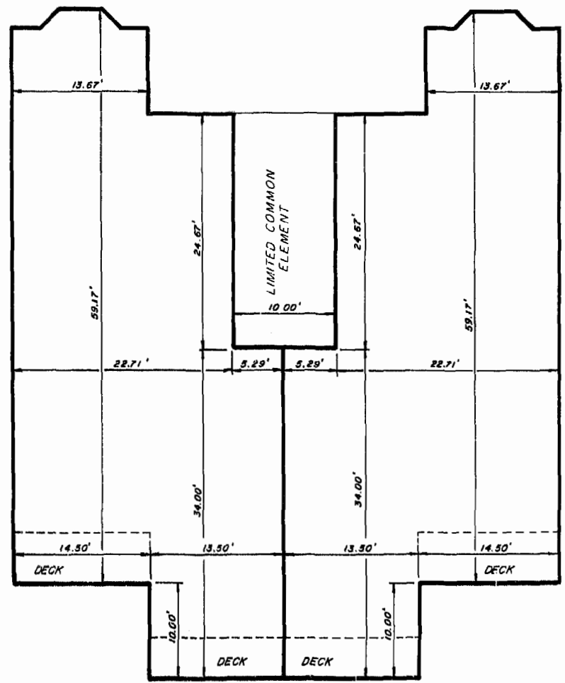
BUILDING 4 SECOND FLOOR UNIT 718 1401 SQ. FT. UNIT 719 1401 SQ. FT. SEE EXHIBIT B FOR VERTICAL BOUNDARY.
