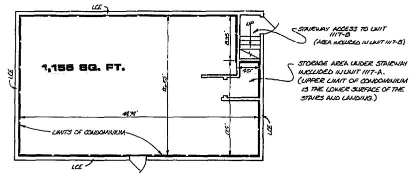
FIRST FLOOR - UNIT 1117-A
