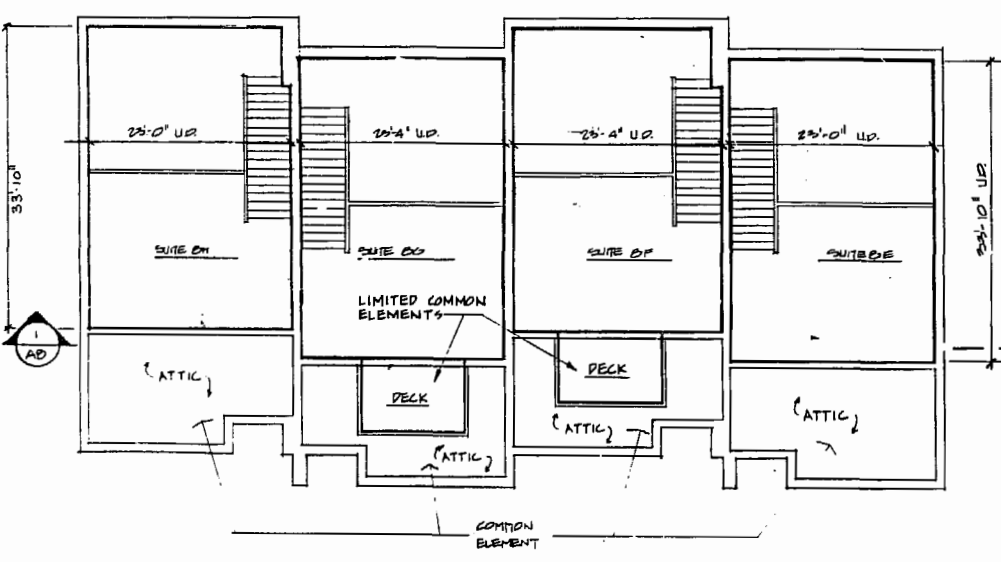
2 LOFT FLOOR PLAN SCALE: 1/8" = 1'-0"
