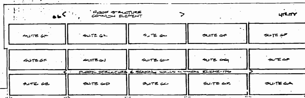
2 FLOOR SECTION 1/8" = 1'-0"
