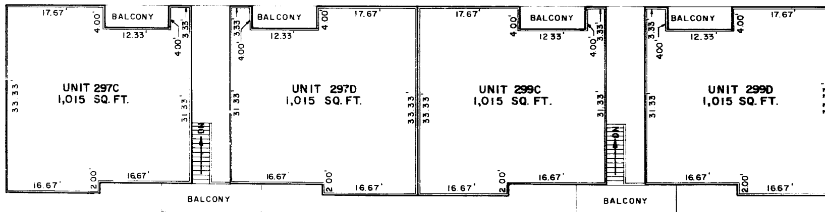
SECOND FLOOR
