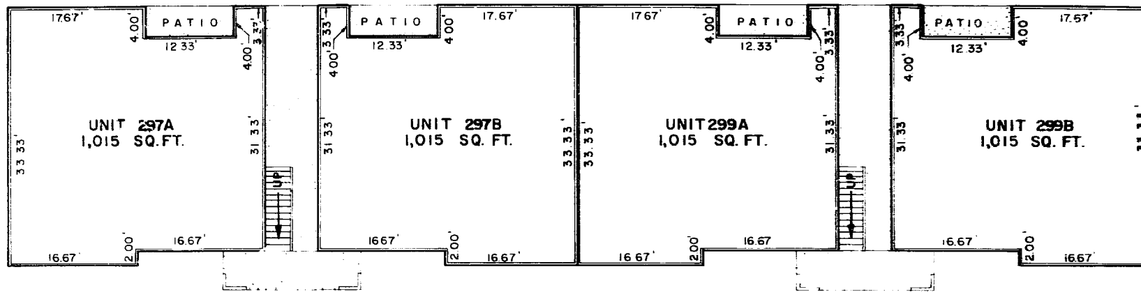
FIRST FLOOR
