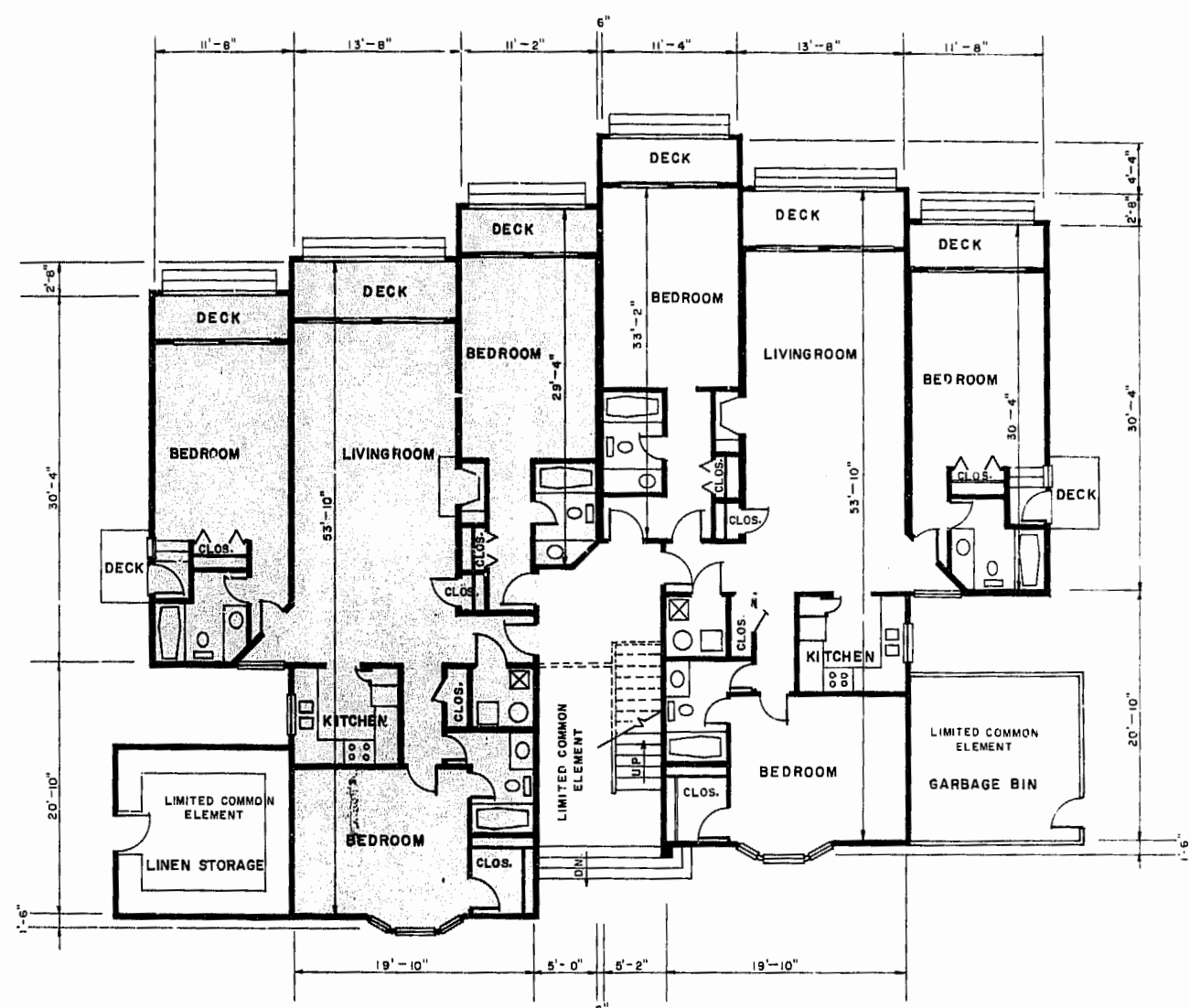
UNIT 116 AREA=1596 SQ. FT.
