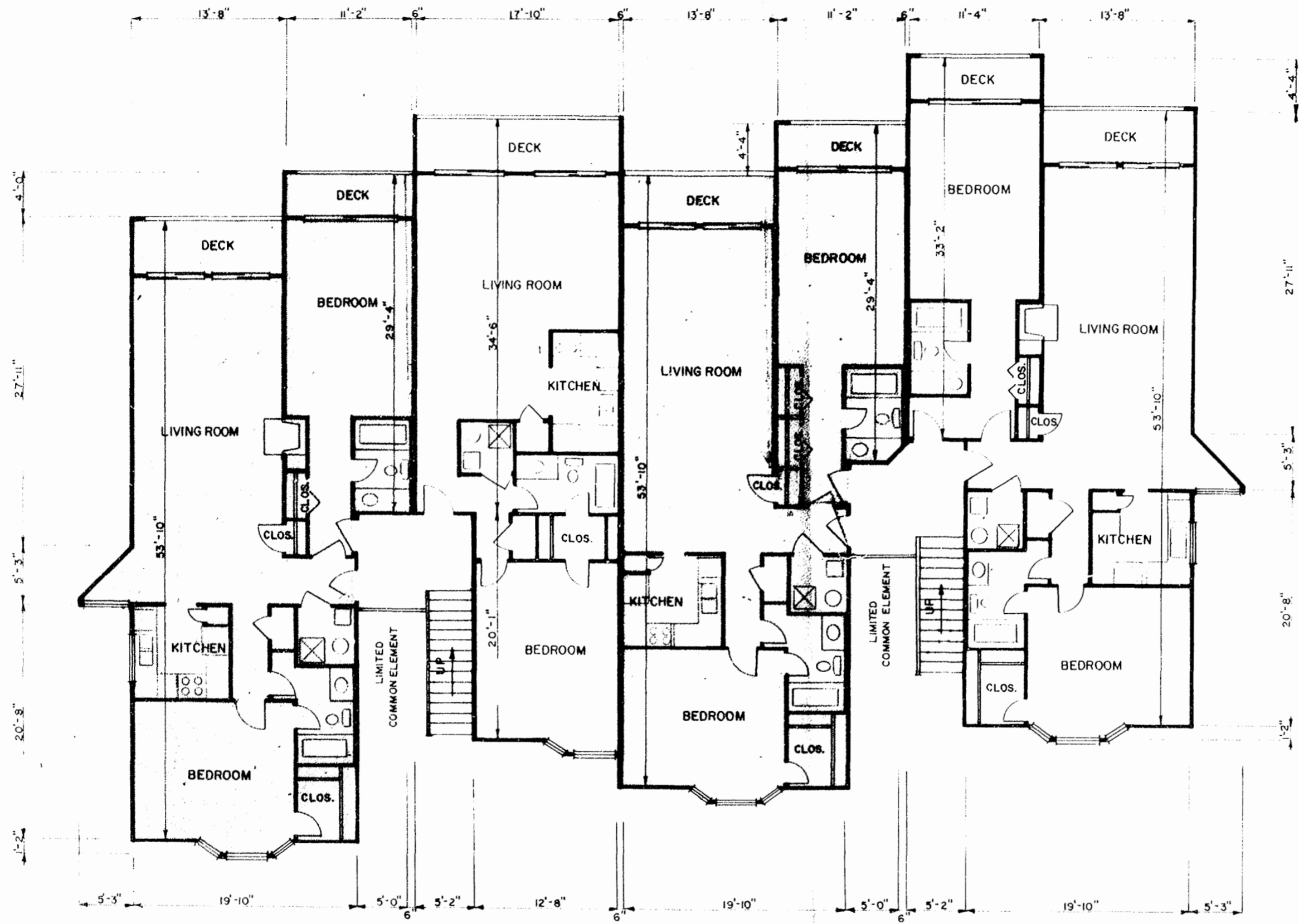
UNIT 101 AREA=1254 SQ.FT.
