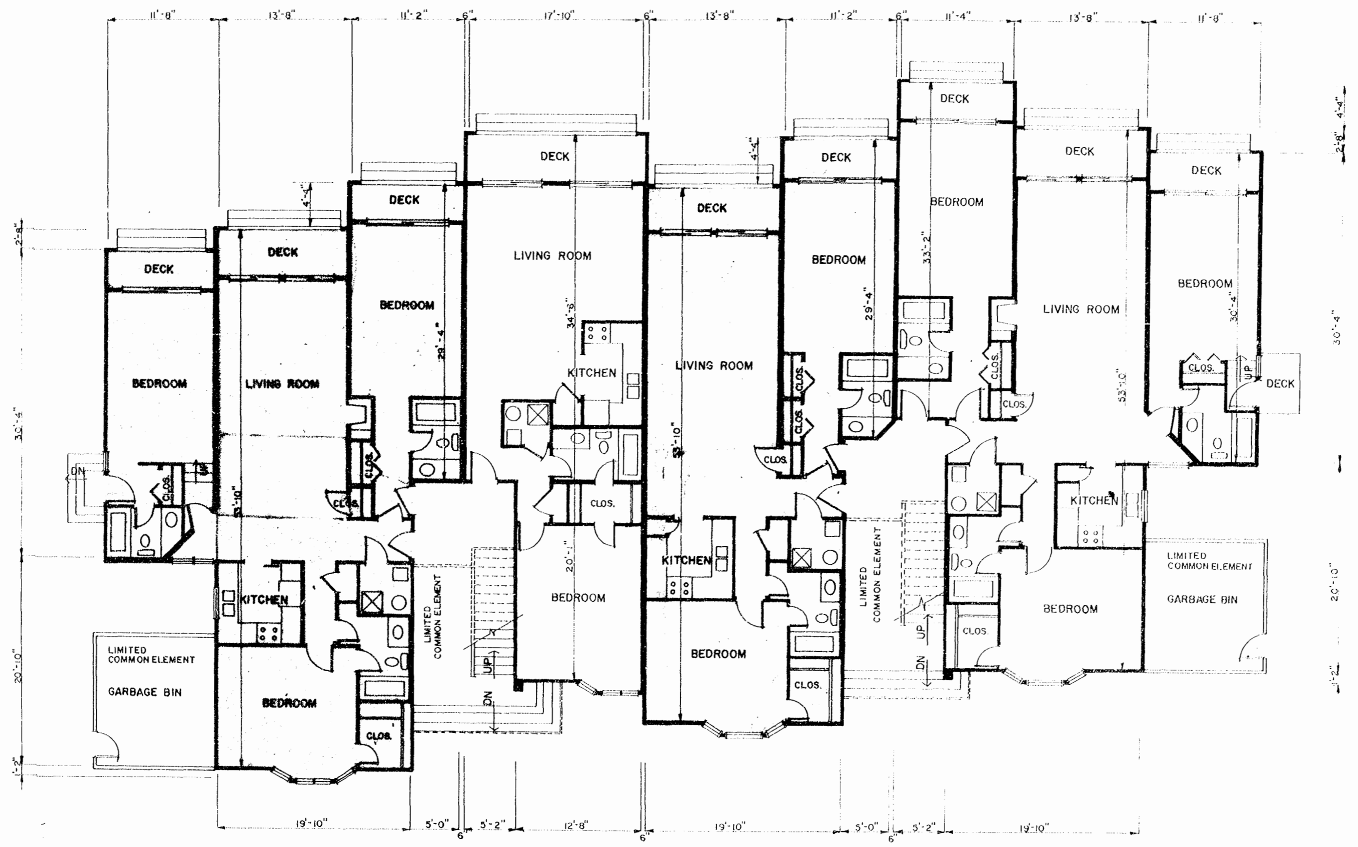
UNIT 100 AREA=1596 SQ. FT.
