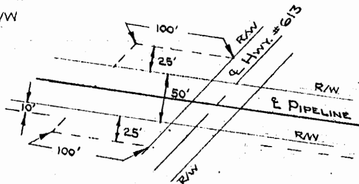
DETAIL "B" SCALE: 1"=100'
