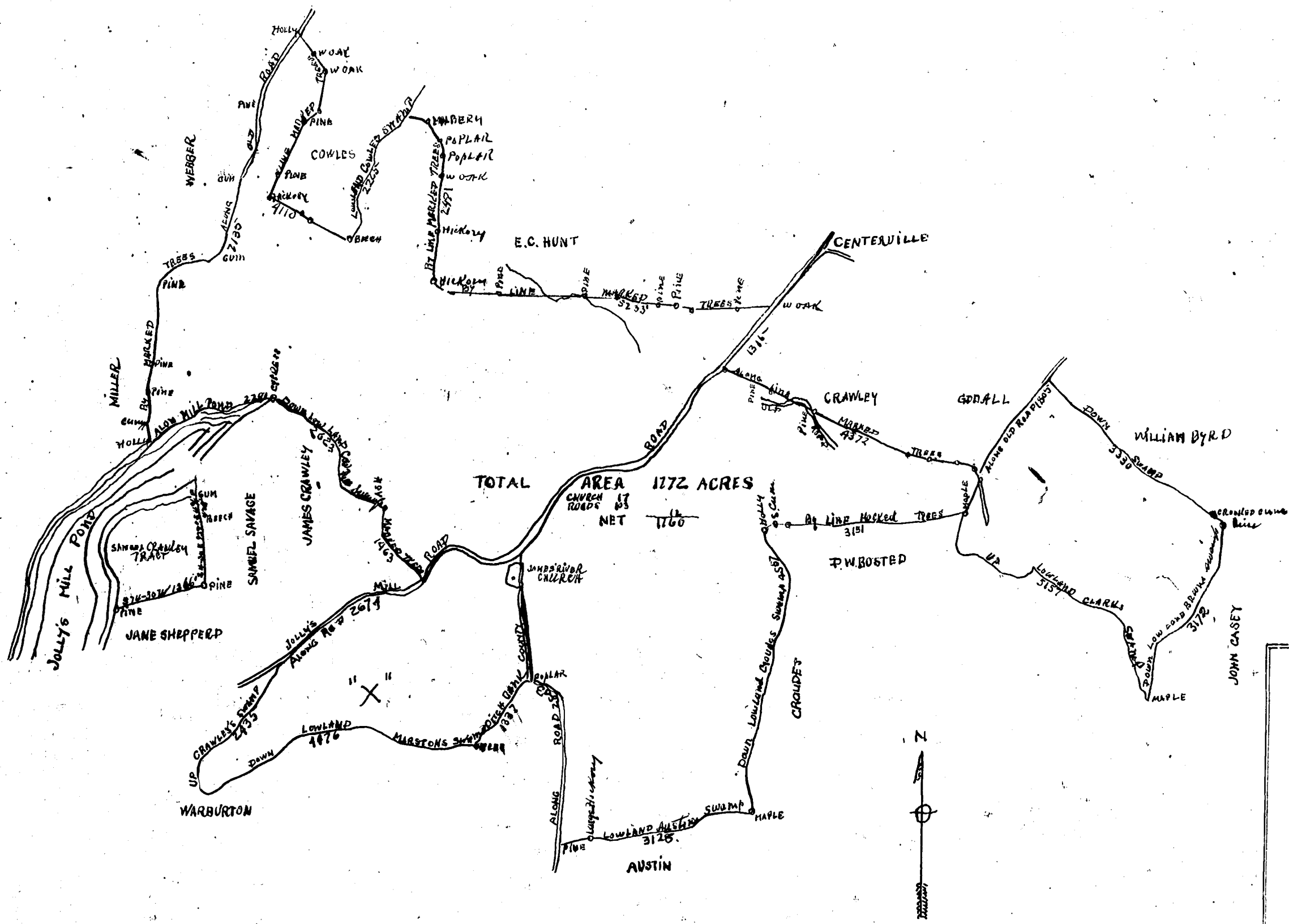
PLAN OF LAND LOCATED IN JAMESTOWN & POWHATAN DISTRICTS, JAMES CITY COUNTY, VIRGINIA, AND KNOWN AS THE SAMUEL CRAWLEY, VANISONS' HOTWATER, CRAWLEYS, MURDOCK, GUNNS, BARTLETTS & CRAMMERS, AND PART OF SUMMER-HOUSE TRACTS SURVEYED AND CALCULATED BY R.H. CLARK, JAMES CITY VA., AUGUST 7, 1914 SCALE ONE INCH TO 1000 FEET
