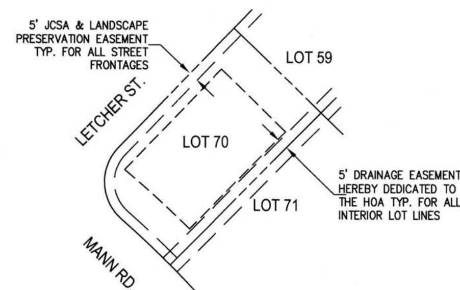
EXHIBIT D TYPICAL DRAINAGE EASEMENTS
