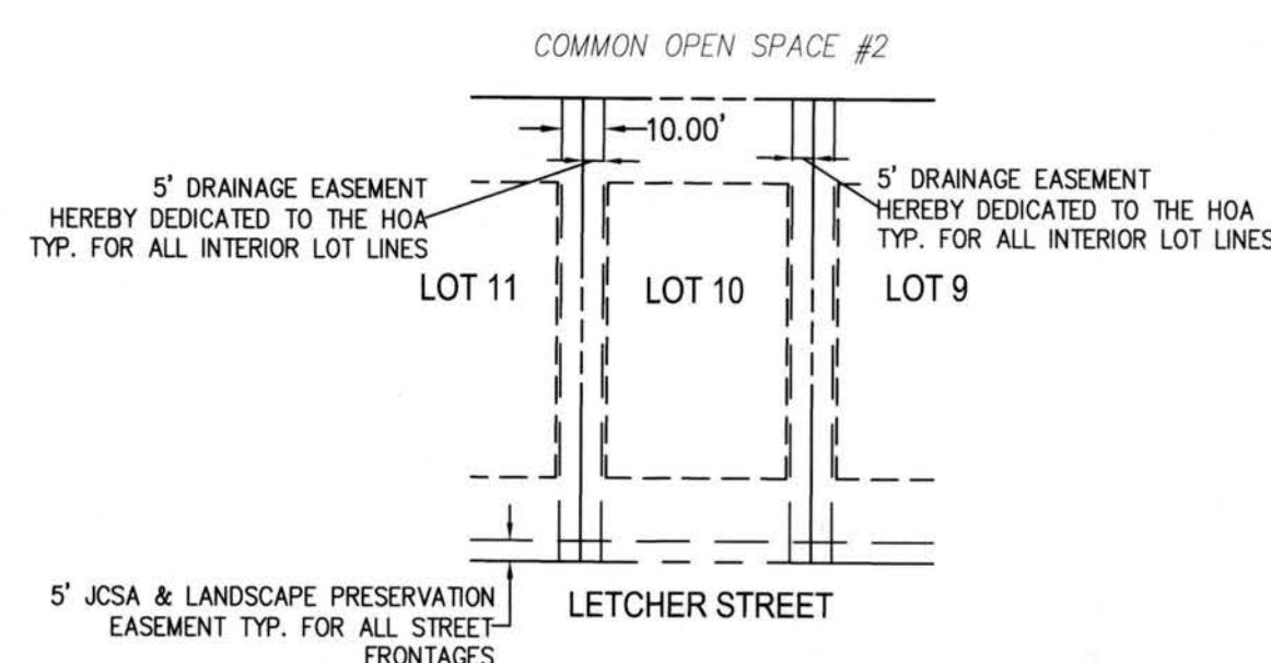
EXHIBIT F TYPICAL DRAINAGE EASEMENTS
