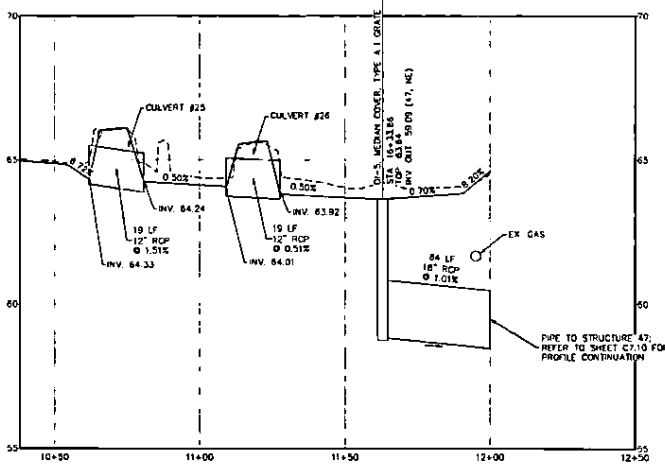
JACKSON STREET WEST STA. 4+80' - 10+25' - Scale: H: 1"=20', V: 10.00:1
