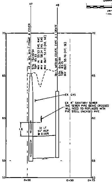
STORM PROFILE 47-48 - Scale: H: 1"=20', V: 10.00:1
