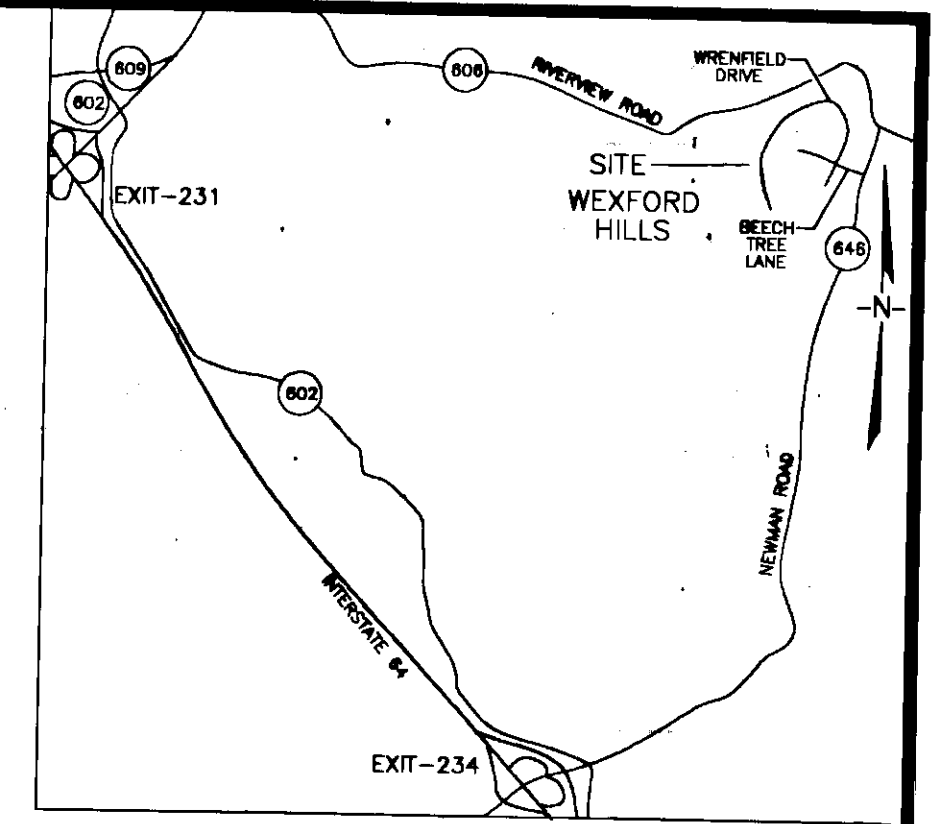
VICINITY MAP
