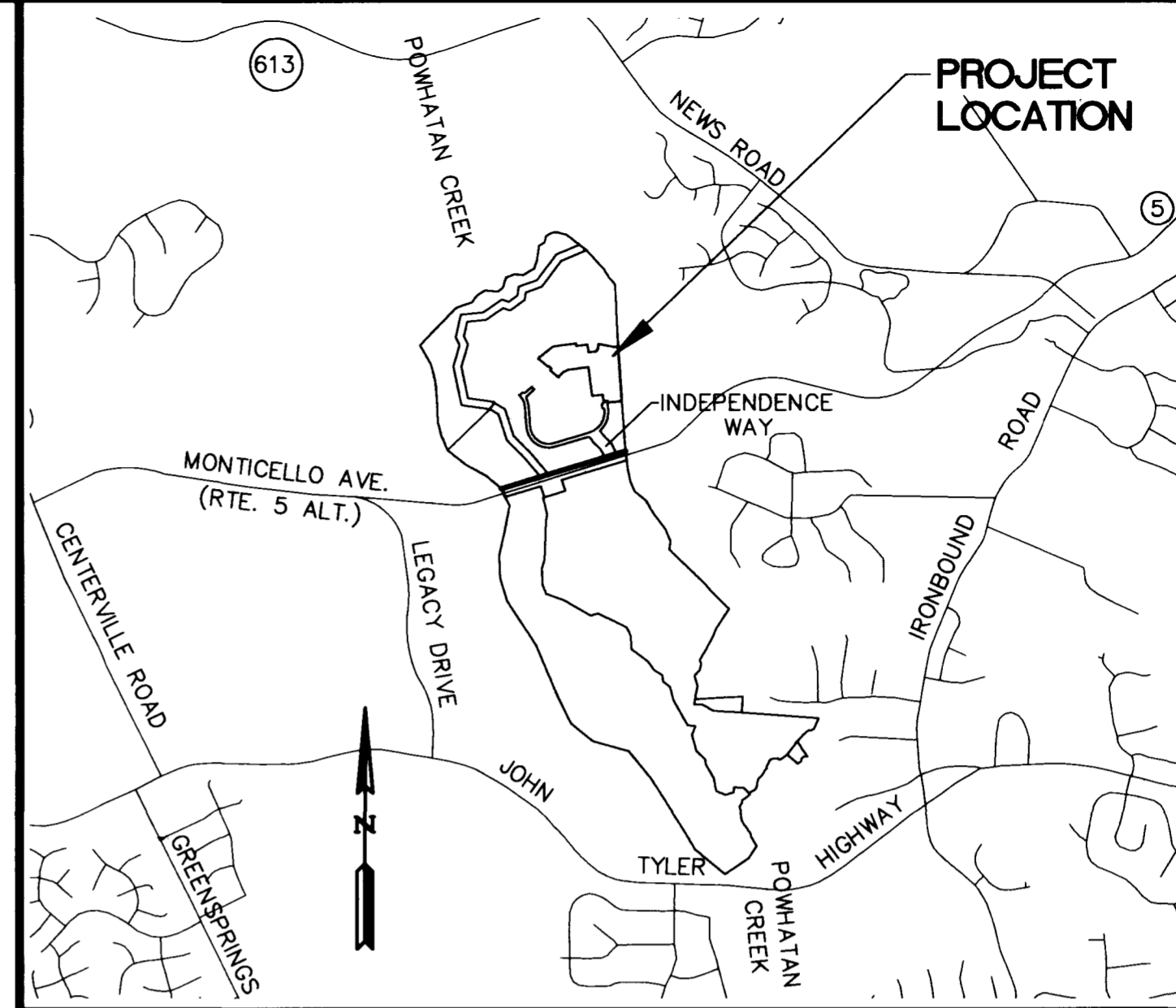
LOCATION MAP
