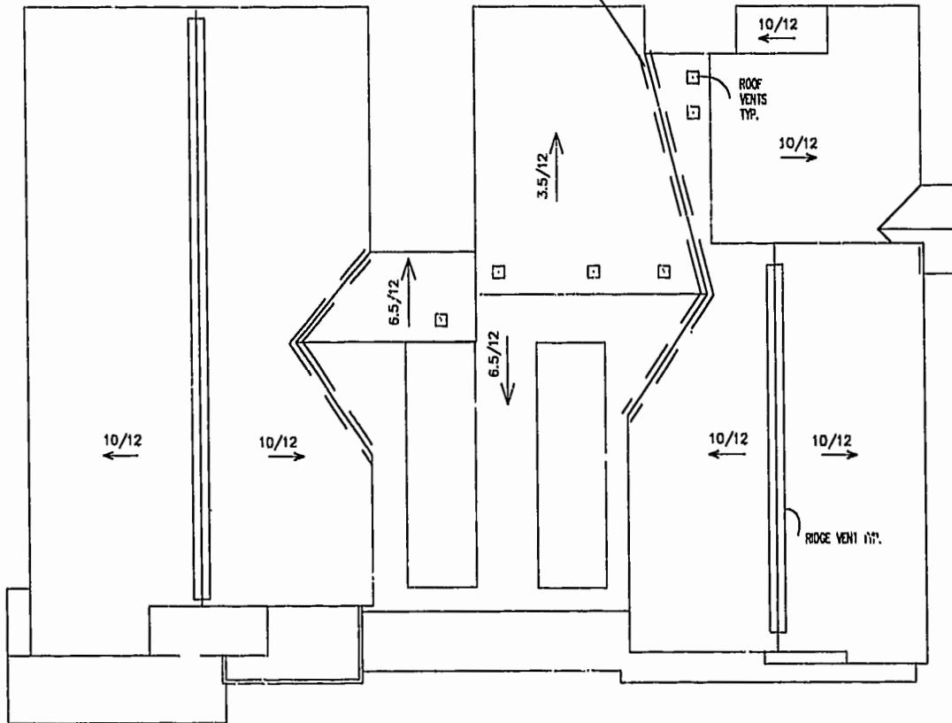
ROOF PLAN
