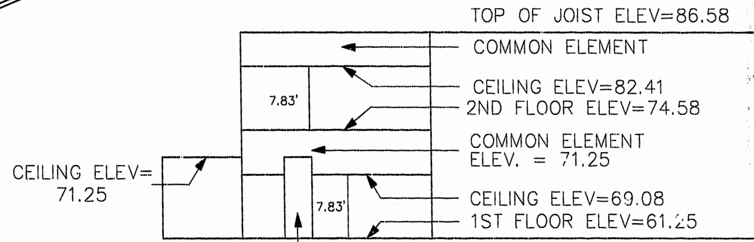
FLOOR ELEVATIONS N.T.S. SECTION AA
