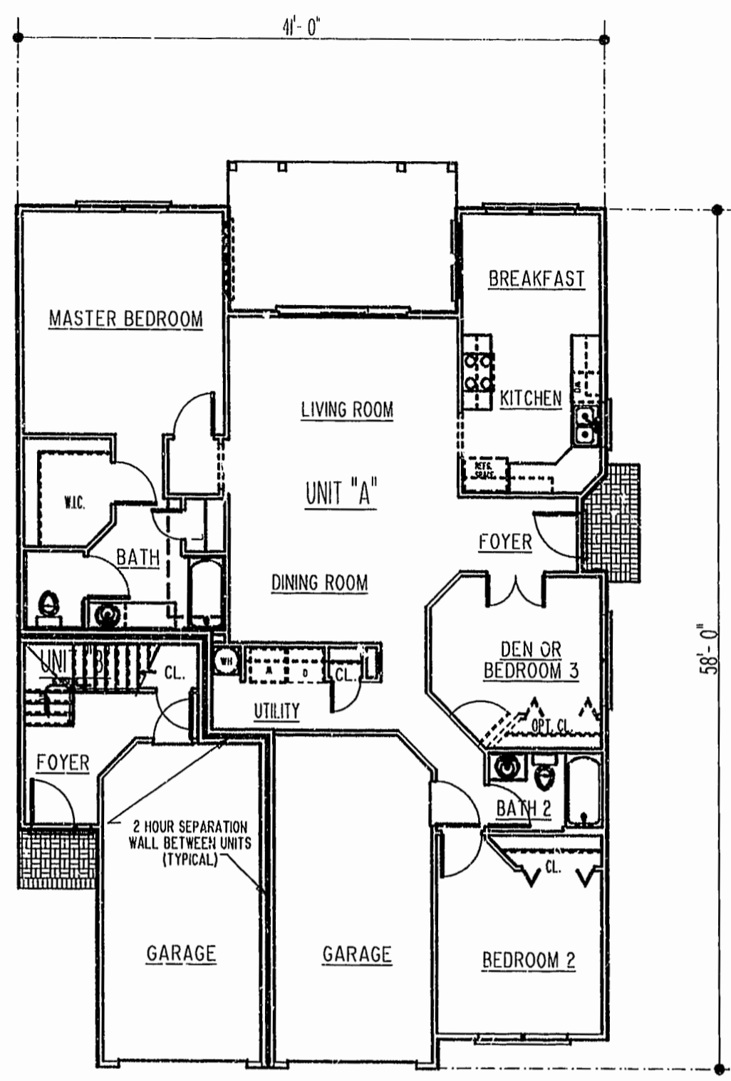
UNIT B ABOVE MODEL 200 "A/B" SCALE: 1/8" = 1'-0"
