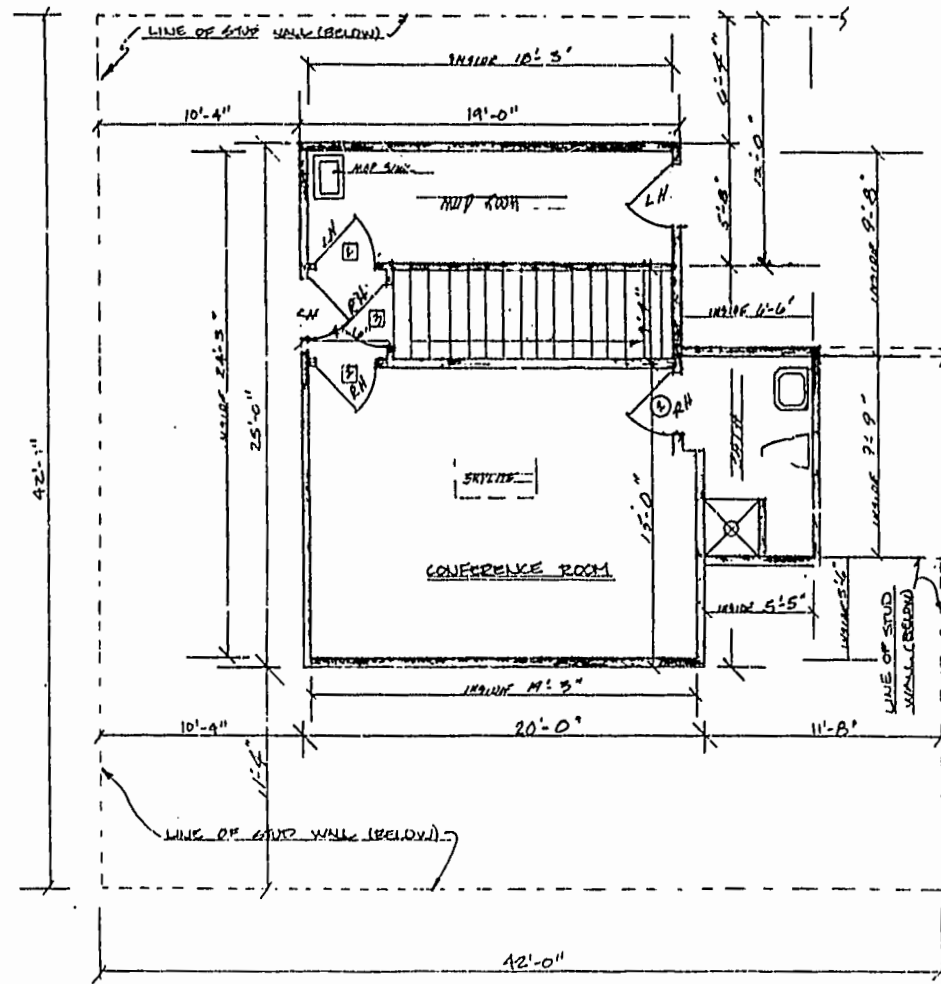
SECOND FLOOR PLAN 1/4" = 1'-0" SQUARE FOOTAGE 1088 SFT.
