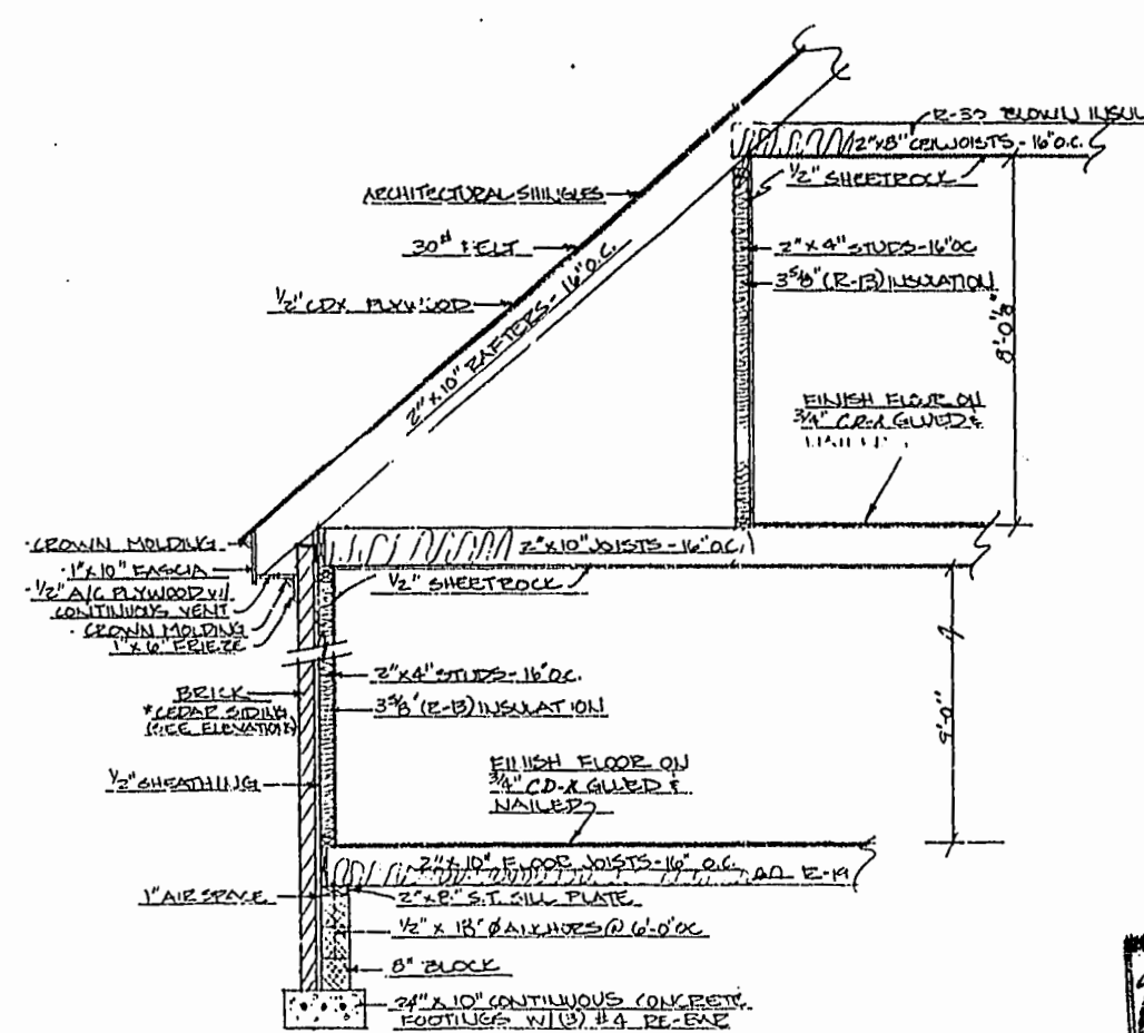
TYPICAL WALL SECTION 1/2" = 1'-0"
