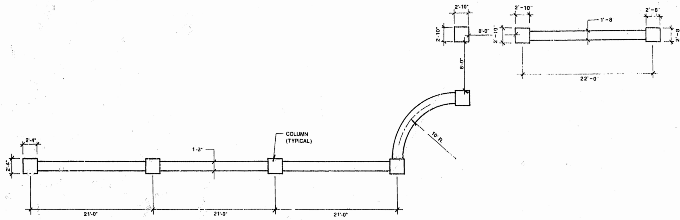
ENTRANCE WALL COMMON ELEMENT (TWO PROVIDED)
