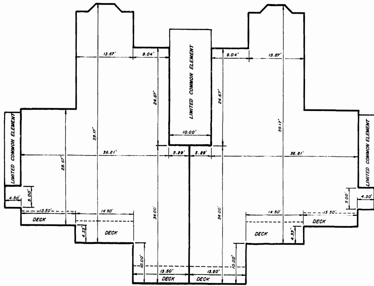
BUILDING 6 SECOND FLOOR SEE EXHIBIT B FOR VERTICAL BOUNDARY.
