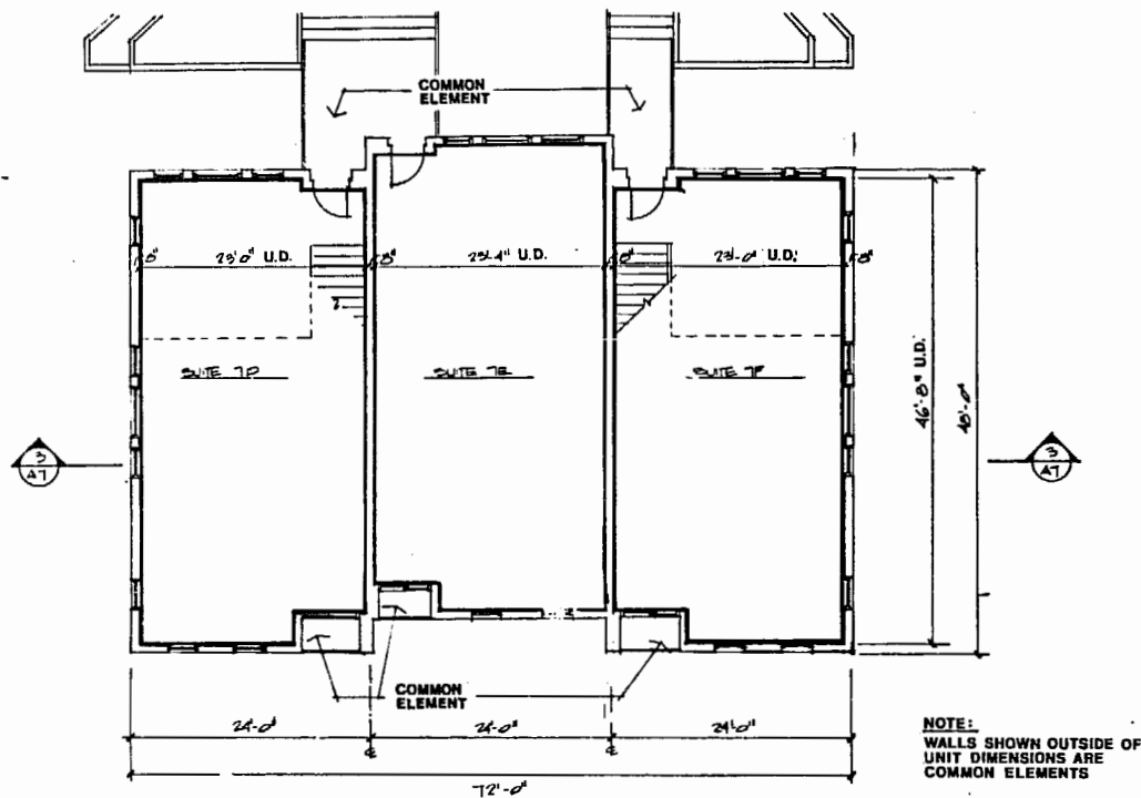
2 SECOND FLOOR PLAN SCALE: 1/8" = 1'-0"
