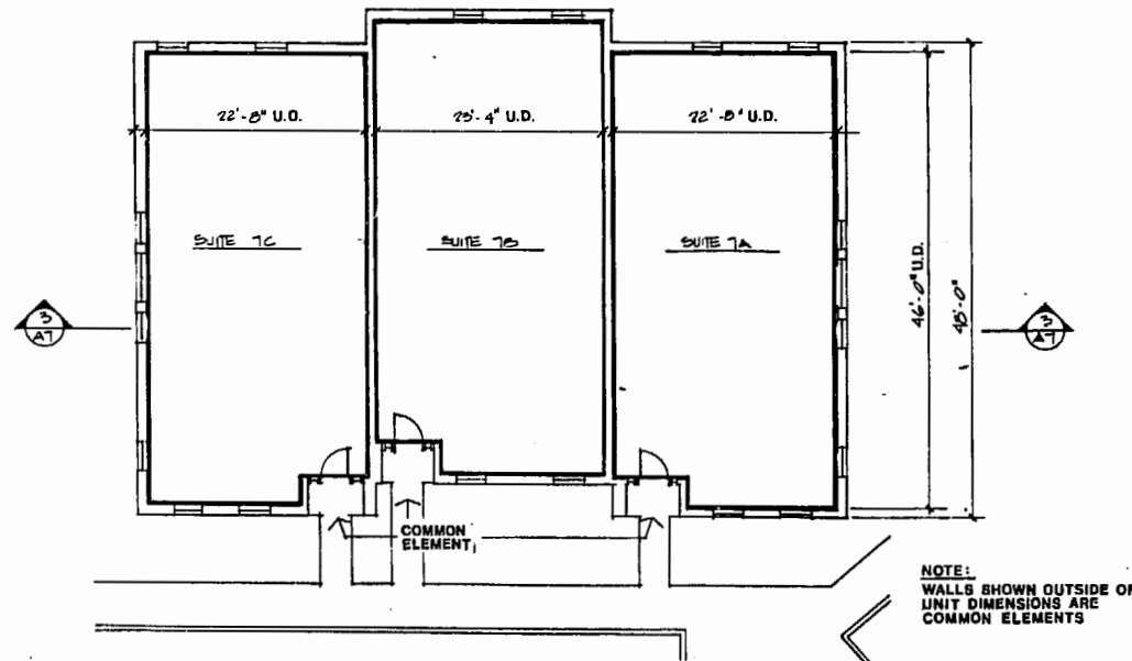
1 FIRST FLOOR PLAN SCALE: 1/8" = 1'-0"
