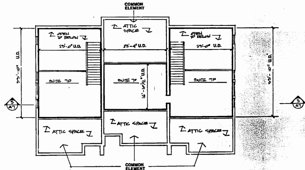
4 LOFT FLOOR PLAN SCALE: 1/8" = 1'-0"
