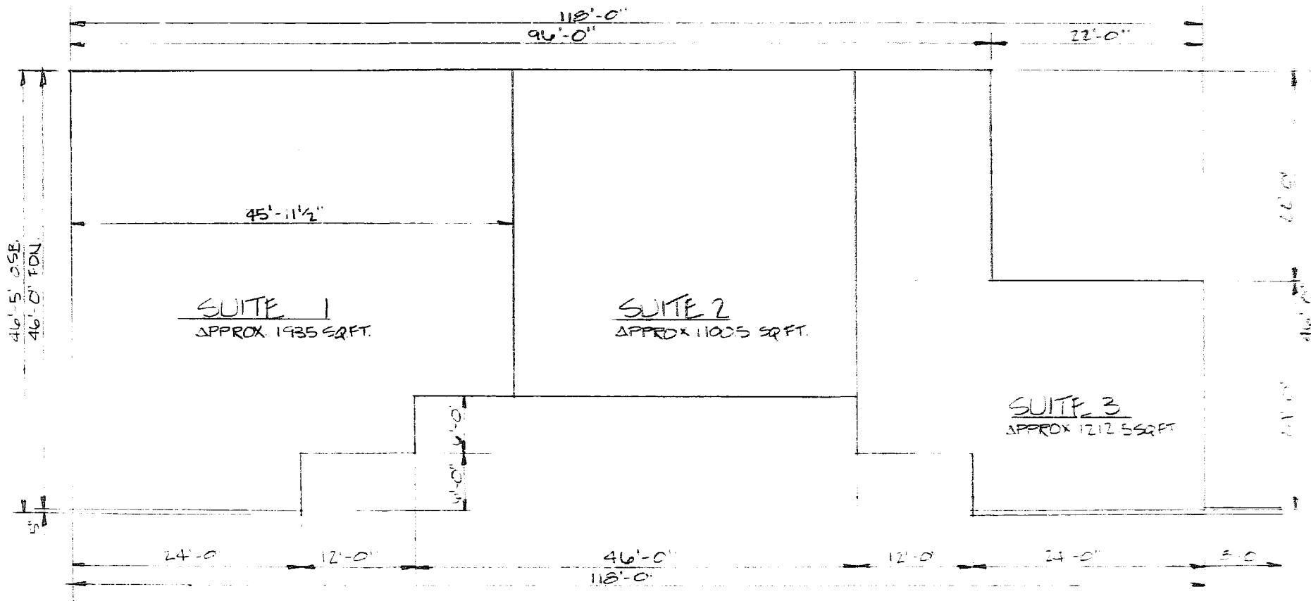
FLOOR PLAN - BUILDING 2 1/8" = 1'-0"
