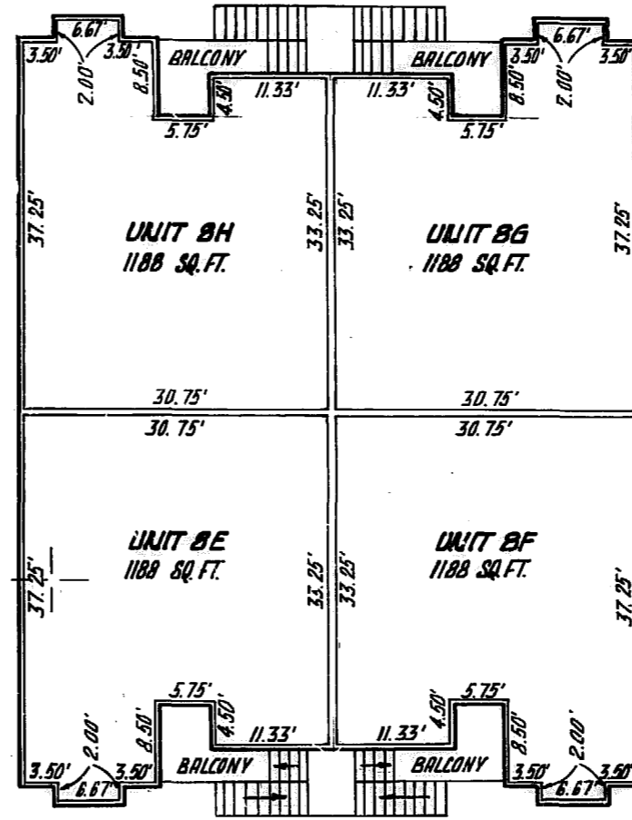
SECOND FLOOR 4 UNITS
