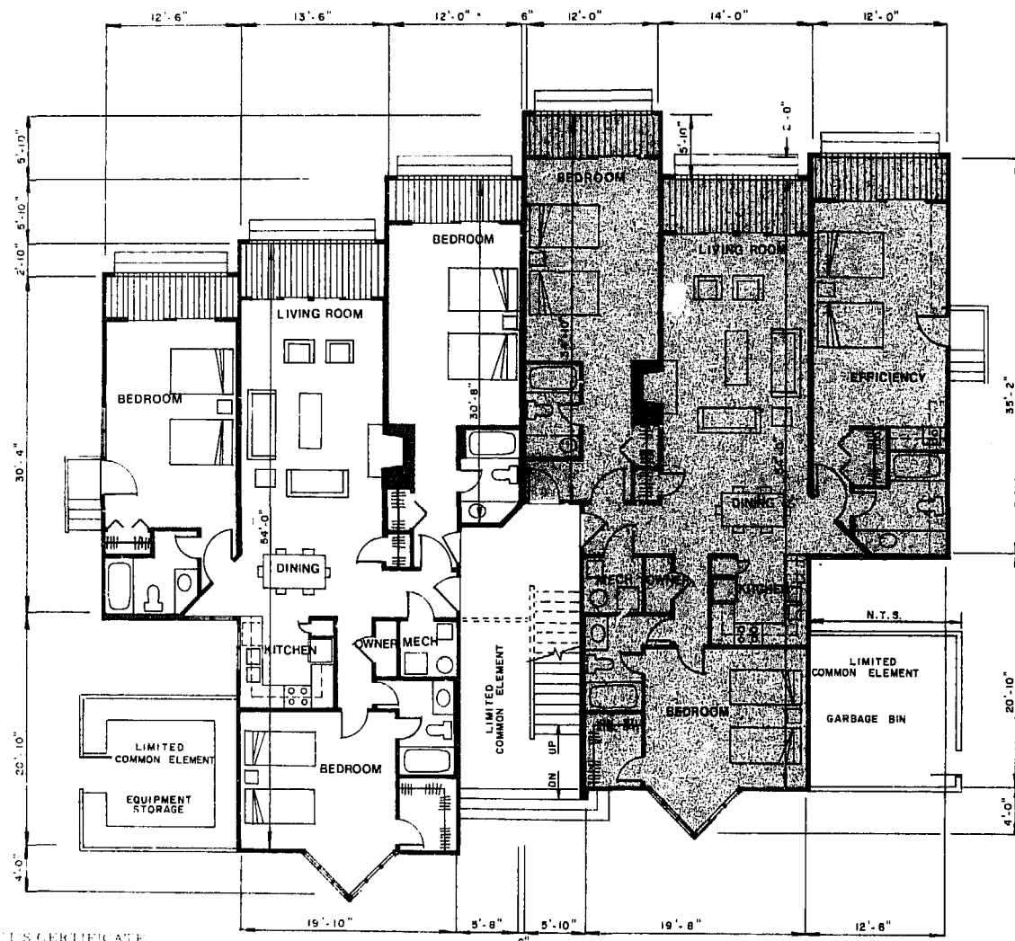
GROUND LEVEL UNIT 200 AREA = 1677 SQ. FT. UNIT 202 AREA = 1757 SQ. FT.
