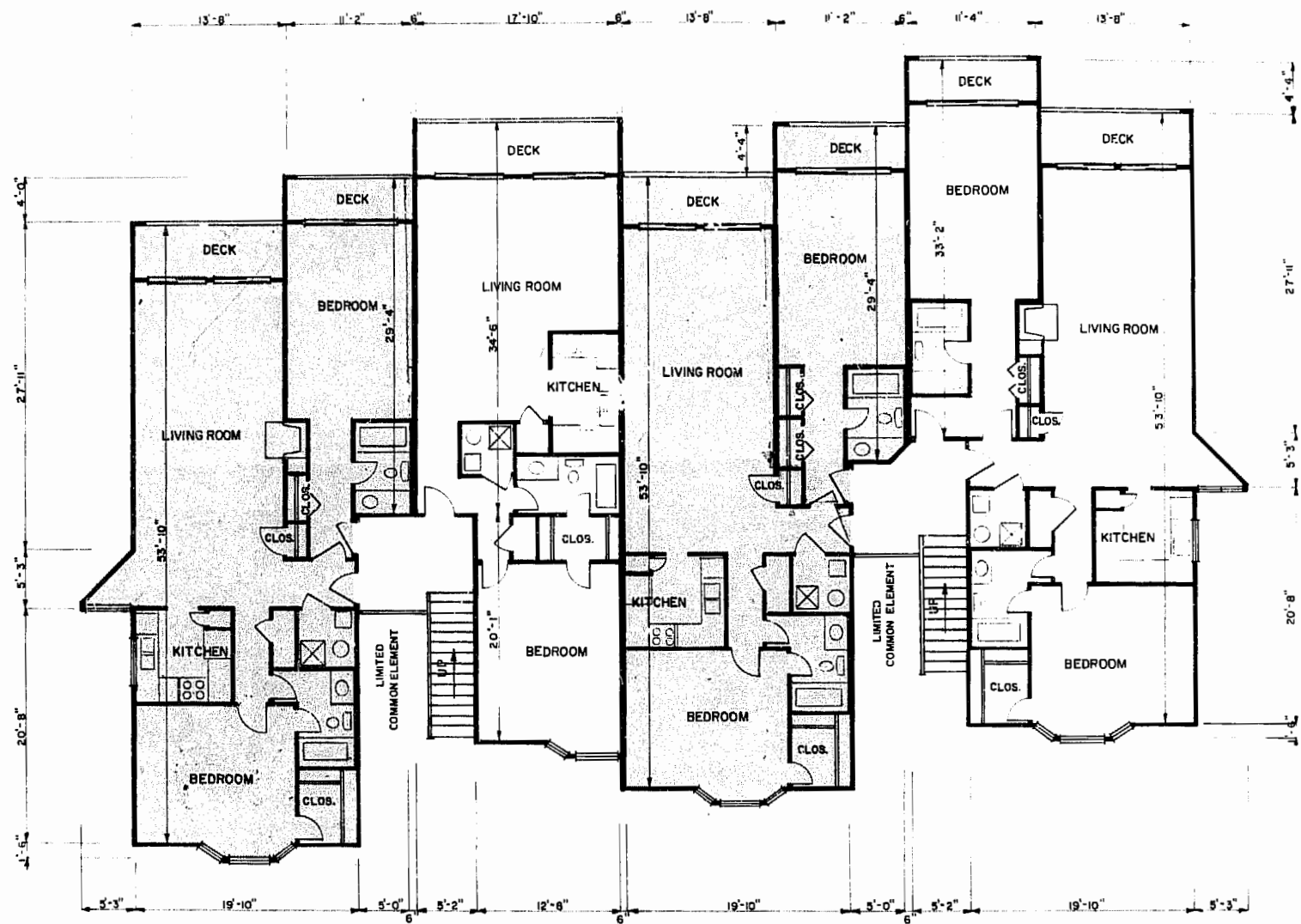
UNIT 129 AREA=1254 SQ.FT.
