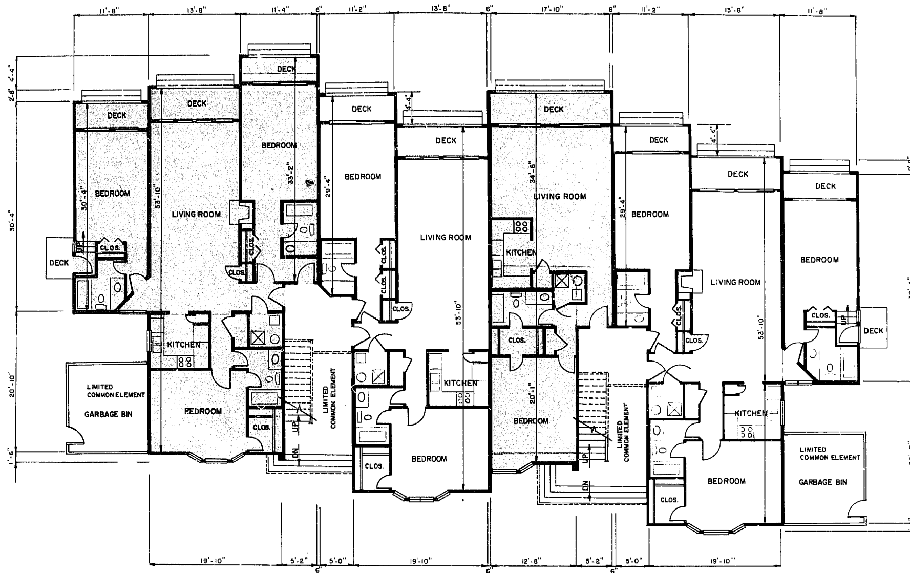
UNIT 120 AREA = 1620 SQ.FT.
