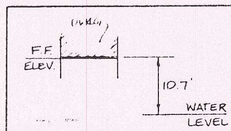
FIRST FLOOR/WATER LEVEL DETAIL
