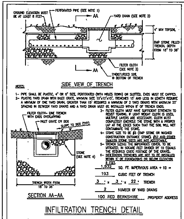
TRENCH DETAIL
