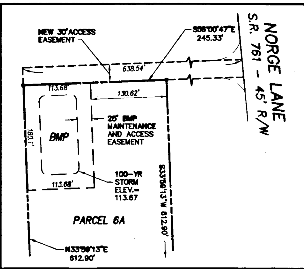
DETAIL FOR BMP EASEMENTS
