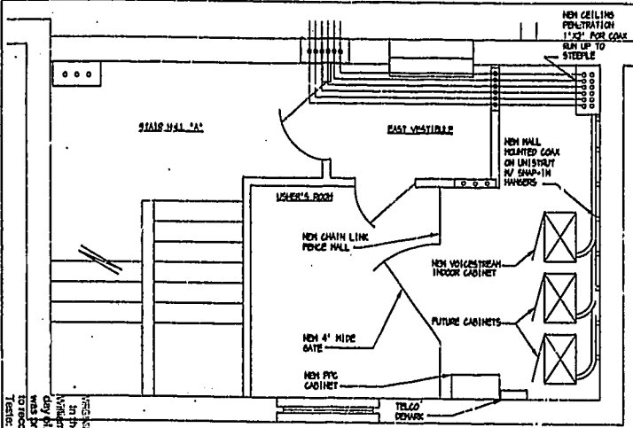
USHER'S ROOM LAYOUT SCALE: 1/4" = 1'
