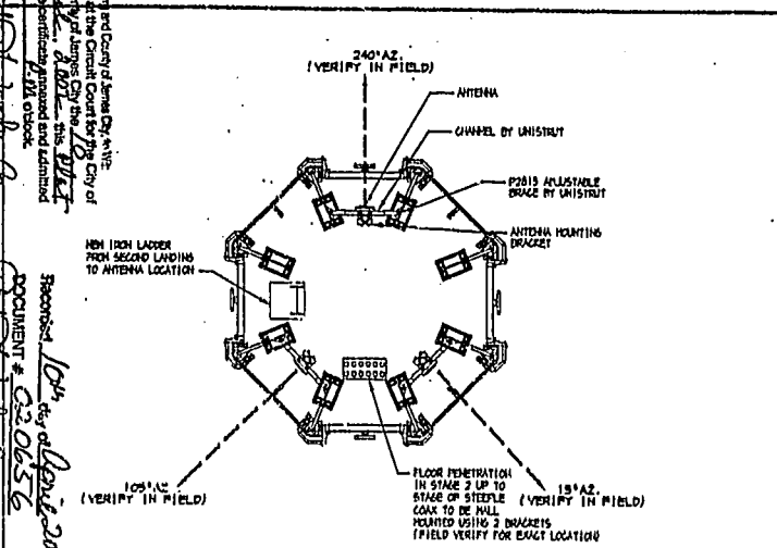
STEEPLE LAYOUT SCALE: 1/4" = 1'
